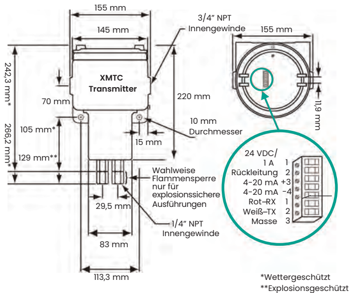
XMTC-Transmitter, Abmessungen
